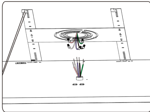
Make proper connections for input and dimming leads Tuck wires into J-box
