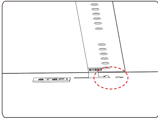
Align bracket plate with luminaire with marking "STEP 1" Slide the luminaire to allow bracket to lock on
