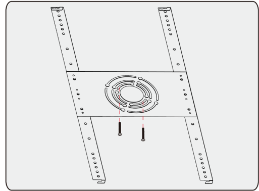
Secure surface mount bracket to ceiling J-box by tighten screws provided
