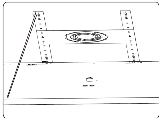
Attach luminaire safety cable to surface mount bracket
